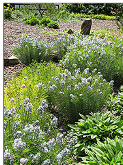
Narrow-Leaf Blue Star in bloom Photo courtesy of NetPS Plant Finder
